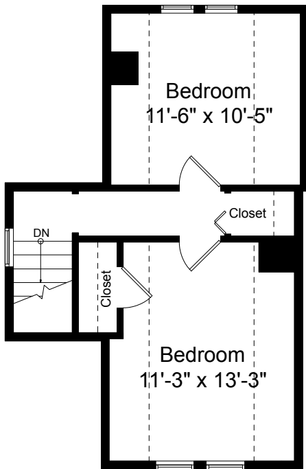
Second Floor Plan Ceiling Height = 7'-0"
